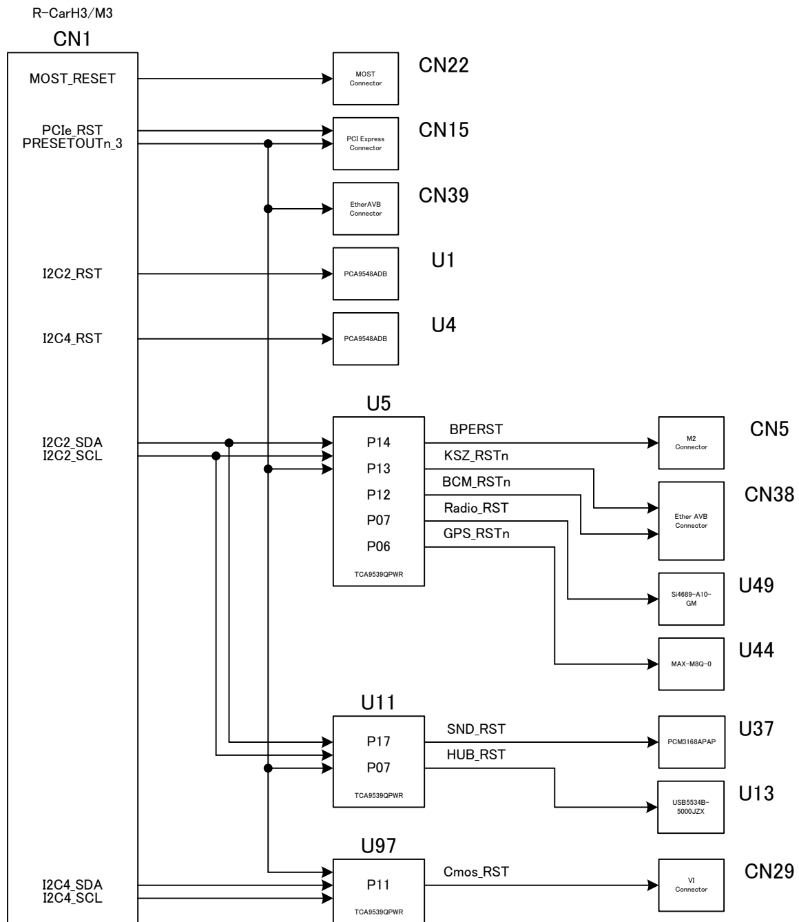
Figure 4-2 : Reset structure
