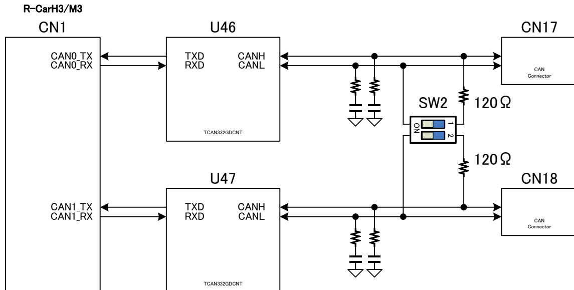
Figure 4-17 CAN I/F
