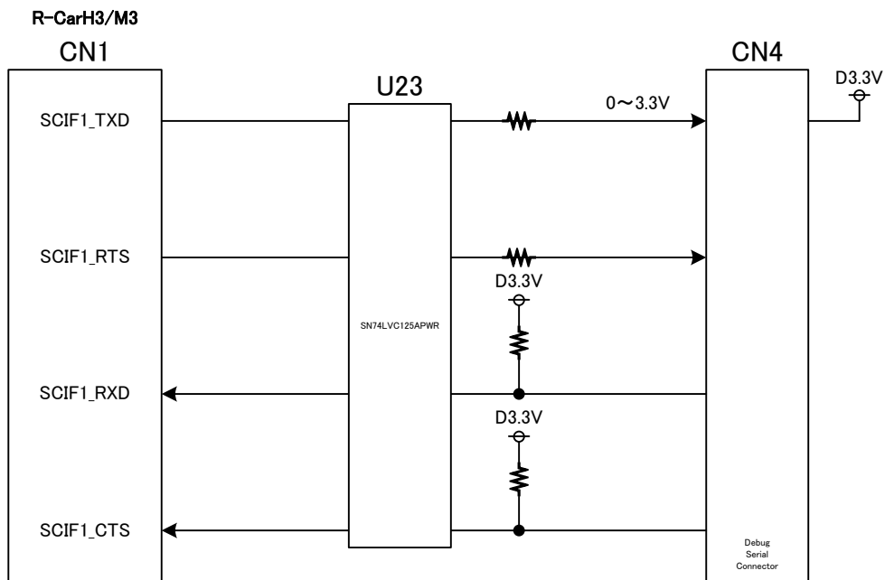
Figure 4-10 : SERIAL I/F
