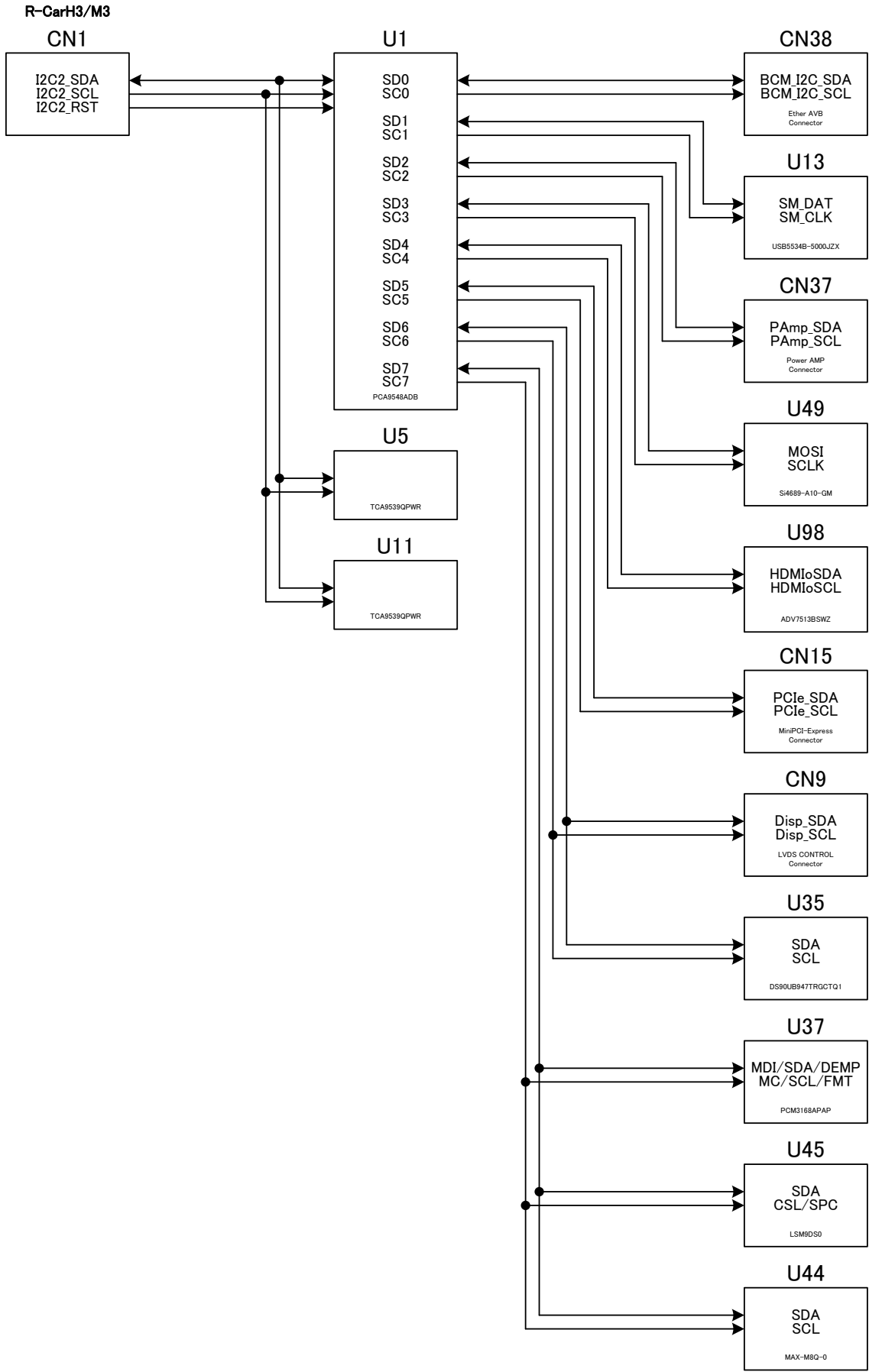
Figure 4-23a : I2C I/F
