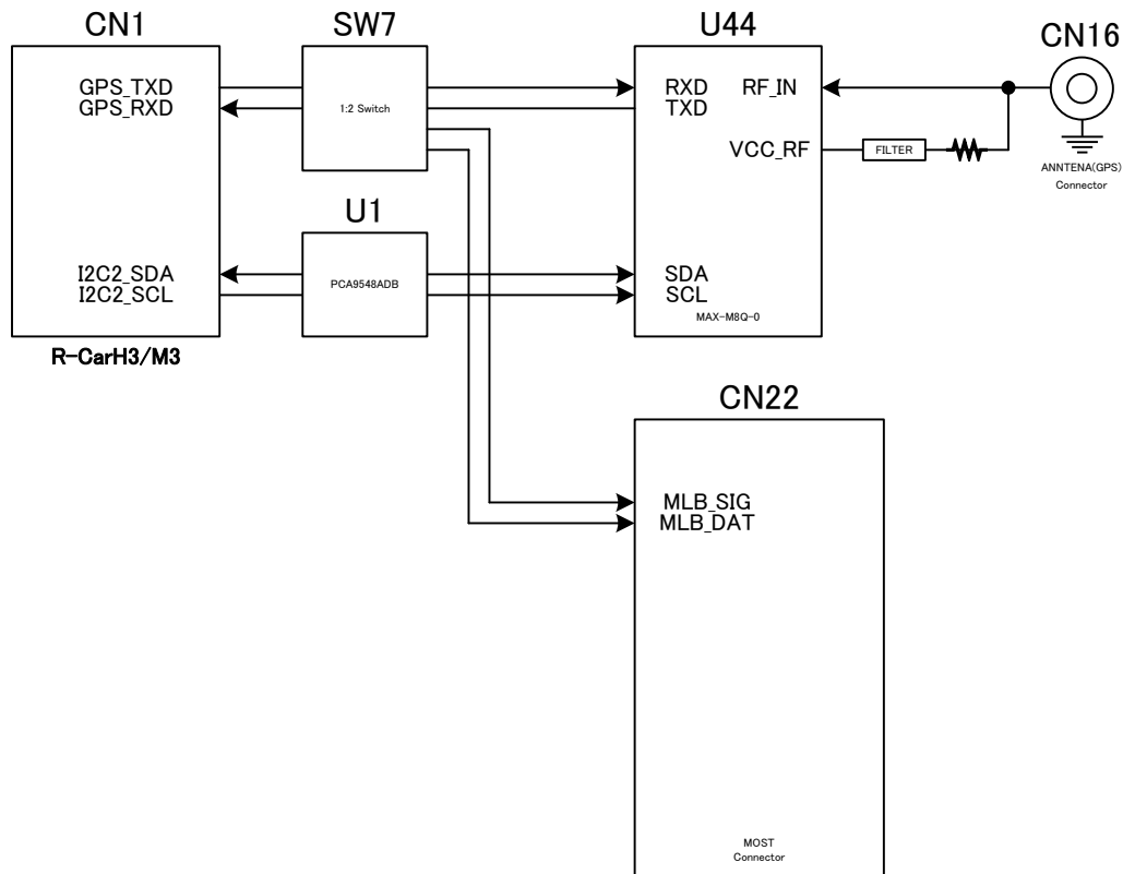
Figure 4-19: GPS I/F
