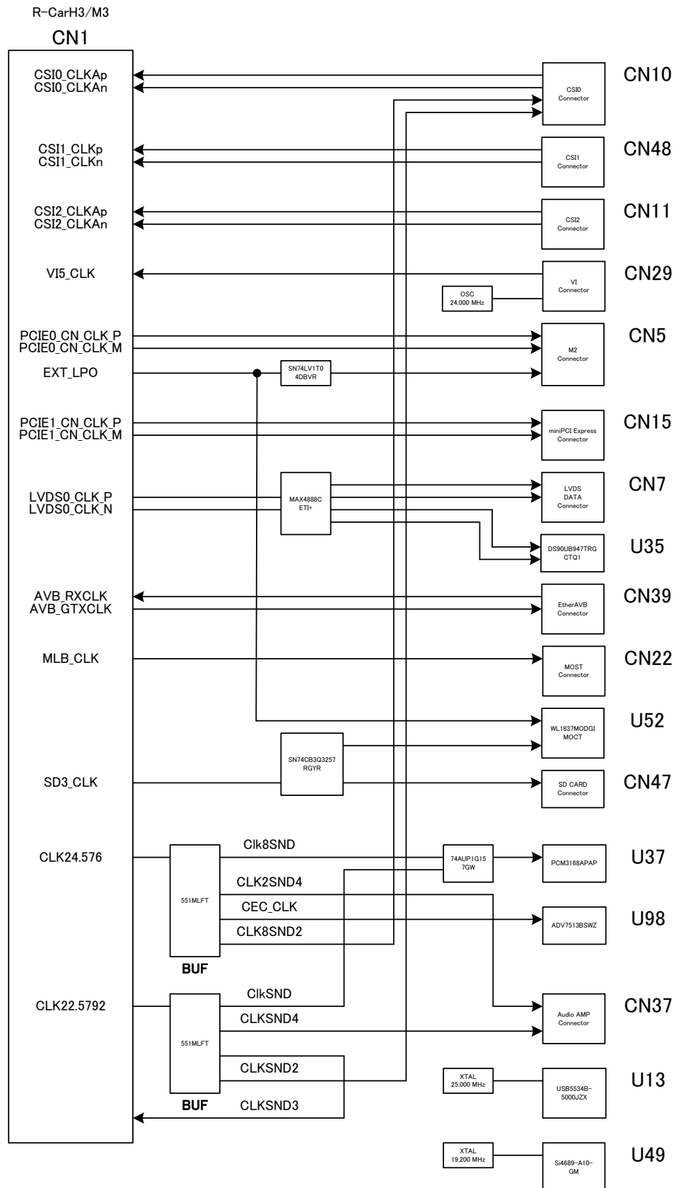
Figure 4-3 : clock structure
