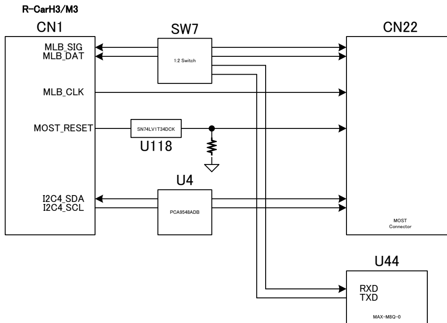
Figure 4-18 : MOST I/F
