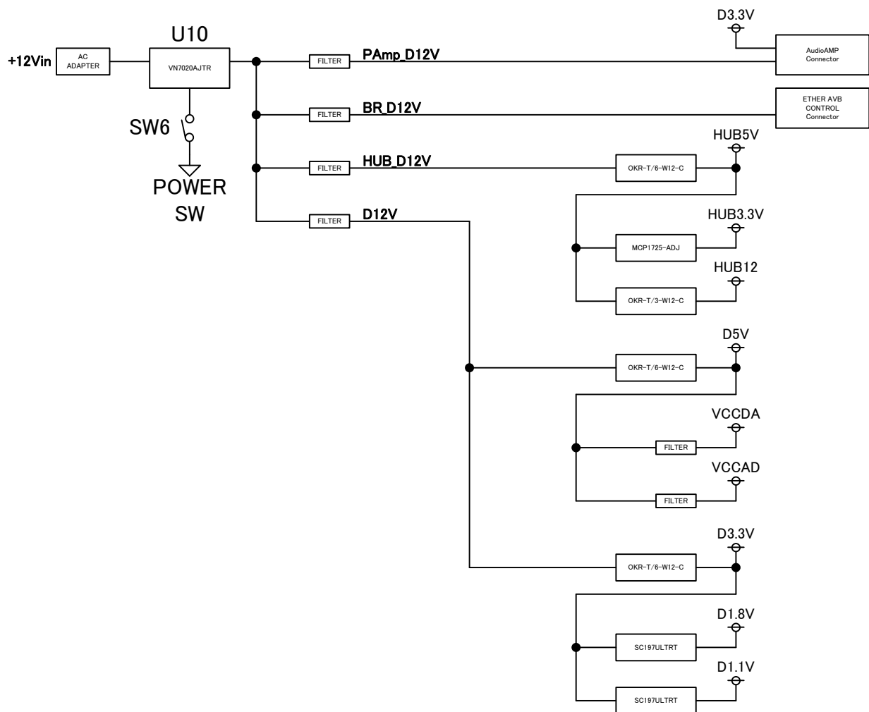
Figure 4-1 : Power structure
