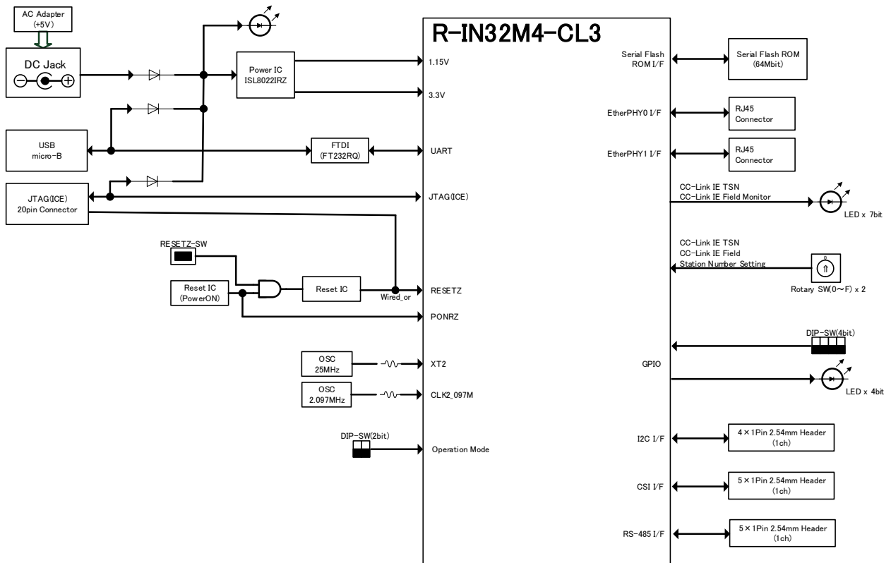
Figure 3 Board Block Diagram
