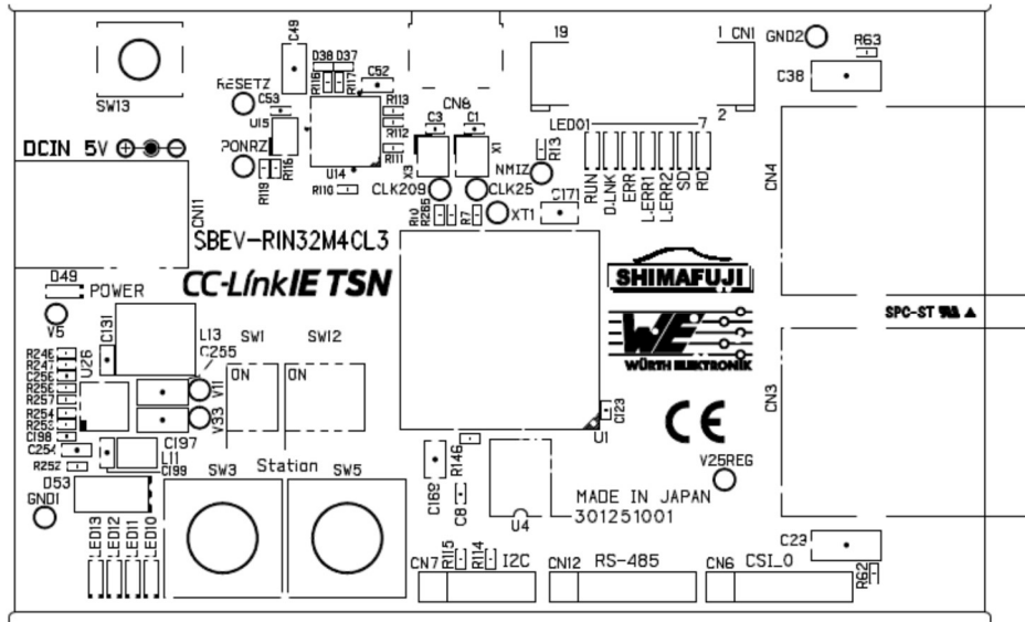
Figure 9a Board Component Side
