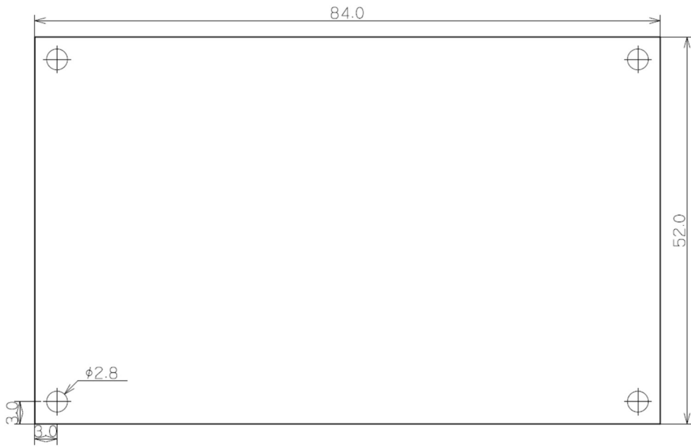
Figure 9c Dimensional
