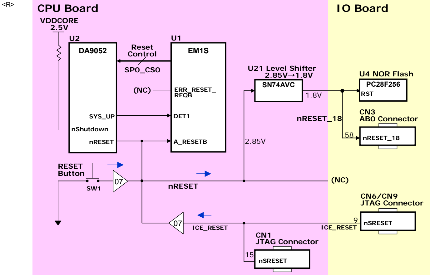
Figure 3-12 Reset System Architecture
